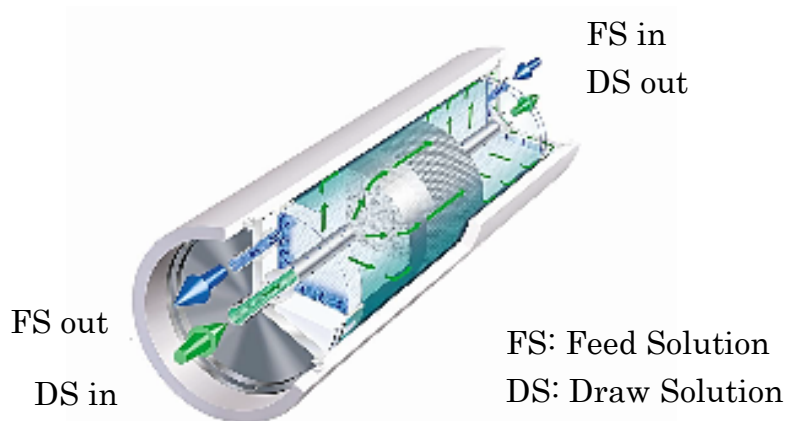
Hollow fiber FO membrane module (schematic diagram)
