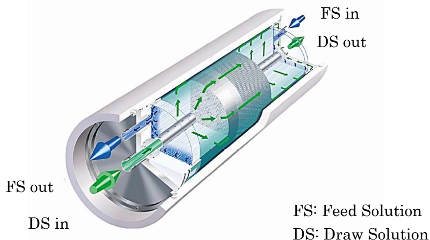
Hollow fiber membrane module for FO (schematic diagram)
